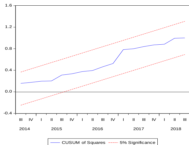
Figure 2: Cumulative Sum of Squares of Recursive Residuals
