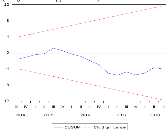
Figure 1: Cumulative Sum of Recursive Residuals
